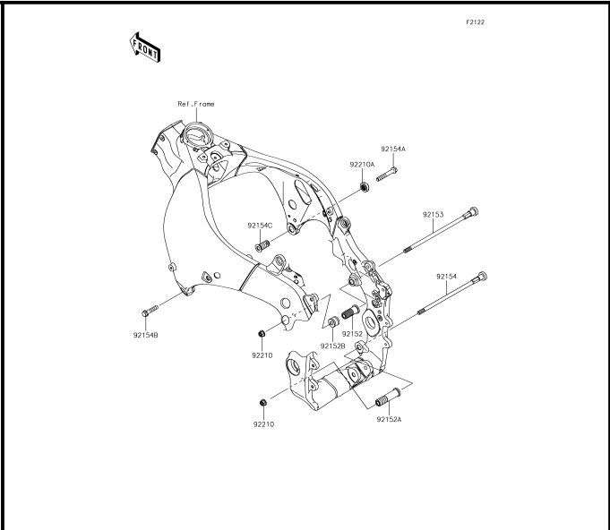
E-4 Engine Mount
