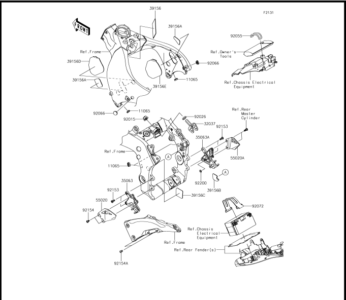
E-5 Frame Fittings
