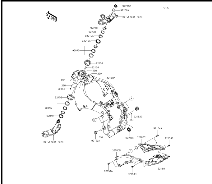
E-3 Frame
